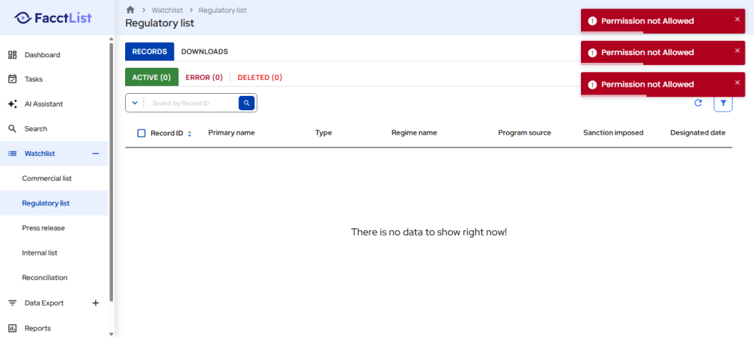
Screenshot: TestExecution_Step56_ACTION_Element.png
