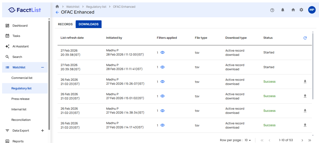
Screenshot: TestExecution_Step37_ACTION_Element.png
