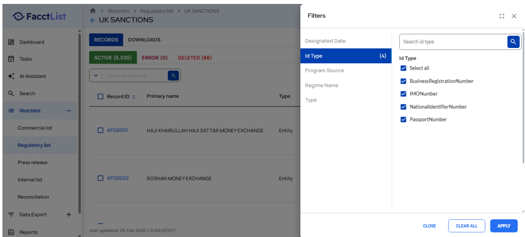
Screenshot: TestExecution_Step51_ACTION_Element.png
