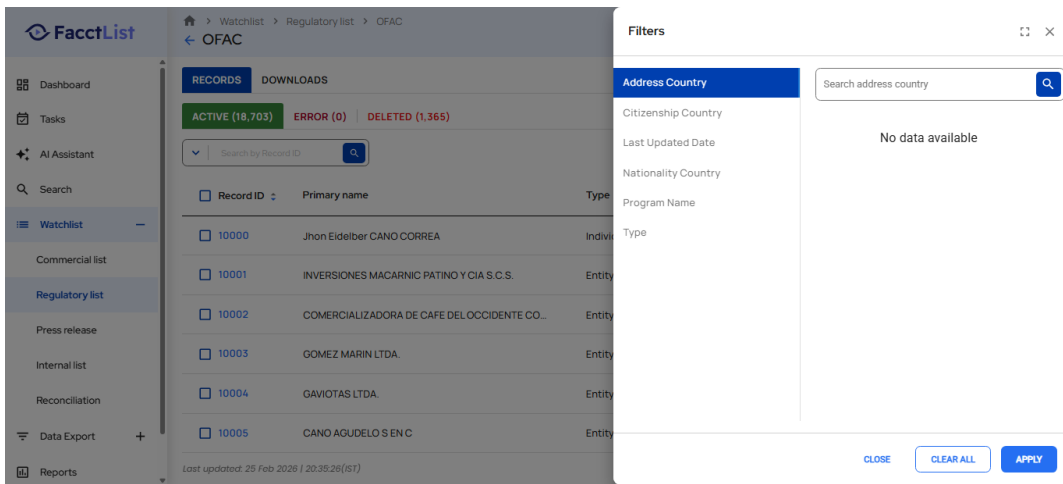
Screenshot: TestExecution_Step32_ACTION_Element.png
