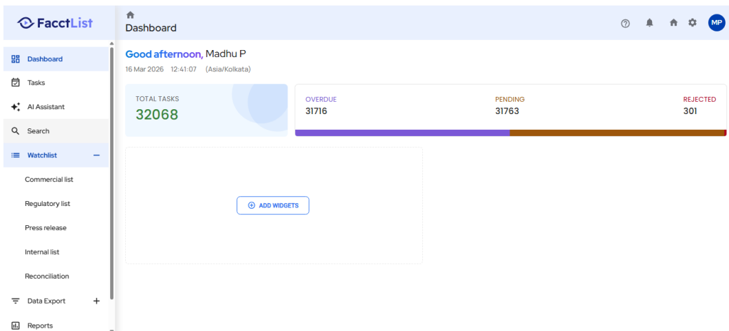
Screenshot: TestExecution_Step54_ACTION_Element.png
