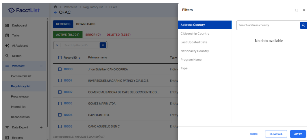
Screenshot: TestExecution_Step35_ACTION_Element.png
