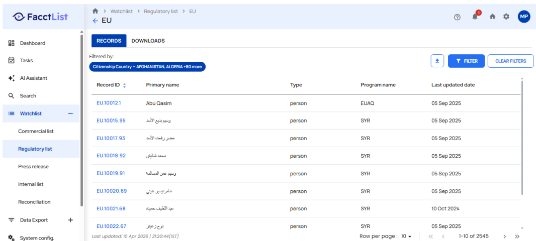
Screenshot: TestExecution_Step03_ACTION_Element.png
