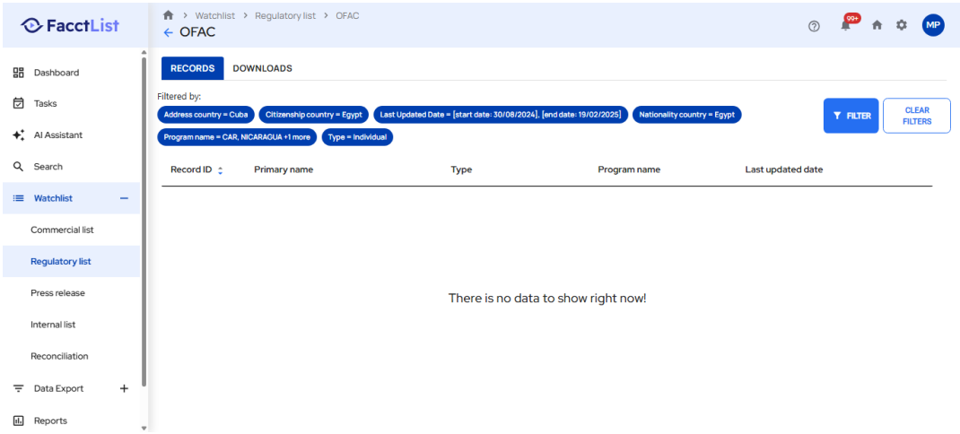
Screenshot: TestExecution_Step09_ACTION_Element.png
