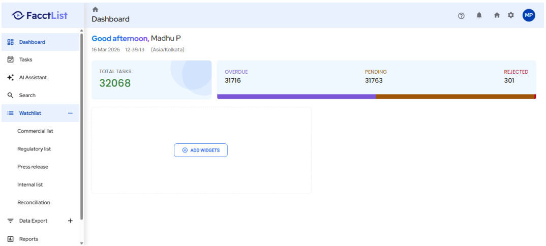
Screenshot: TestExecution_Step60_ACTION_Element.png
