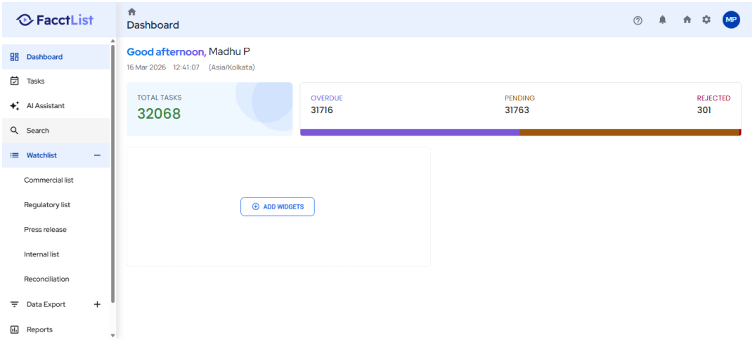
Screenshot: TestExecution_Step61_ACTION_Element.png
