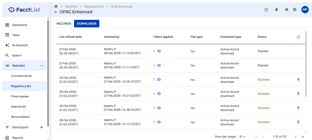
Screenshot: TestExecution_Step44_ACTION_Element.png
