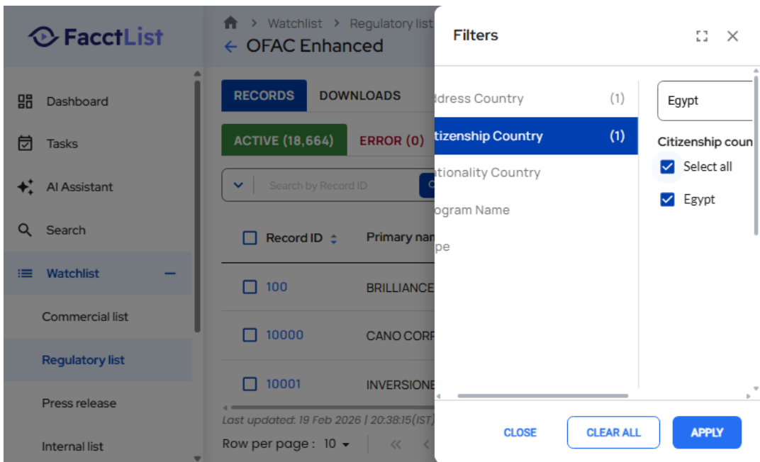
Screenshot: TestExecution_Step19_ACTION_Element.png
