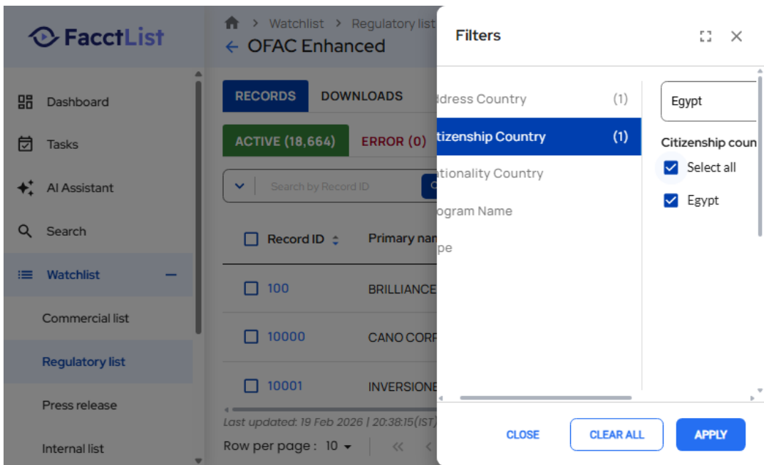
Screenshot: TestExecution_Step18_ACTION_Element.png
