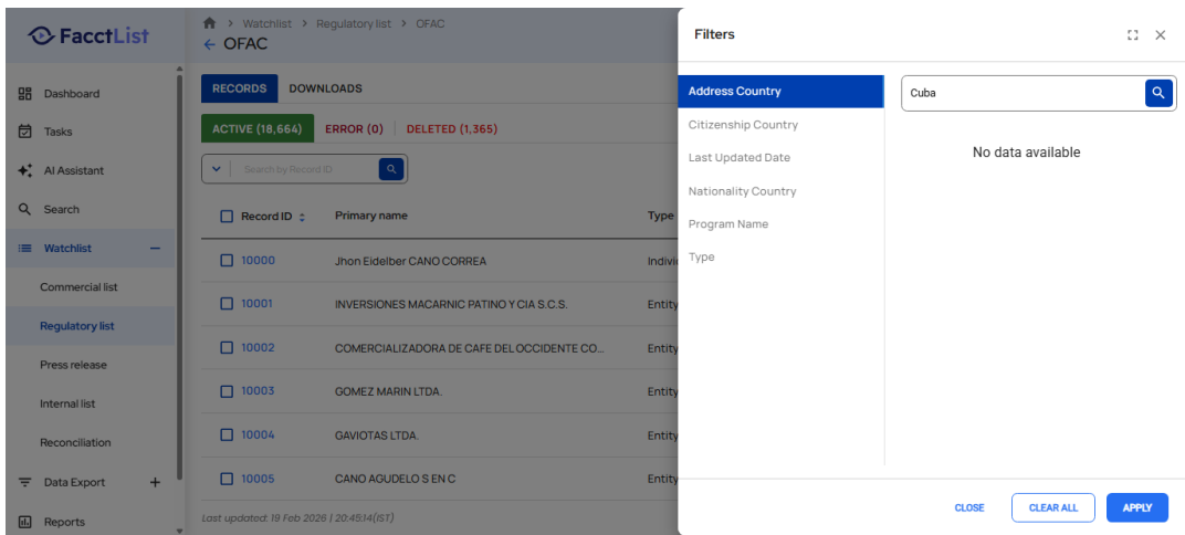
Screenshot: TestExecution_Step17_ACTION_Element.png
