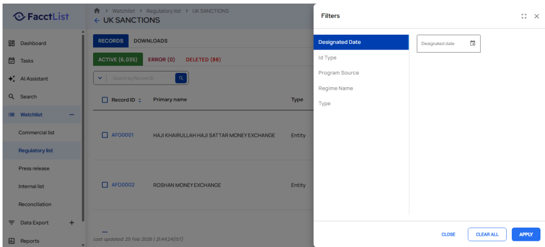
Screenshot: TestExecution_Step57_ACTION_Element.png
