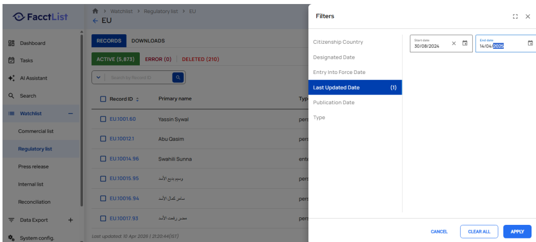
Screenshot: TestExecution_Step04_ACTION_Element.png
