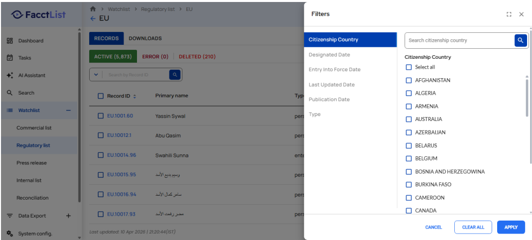
Screenshot: TestExecution_Step01_ACTION_Element.png
