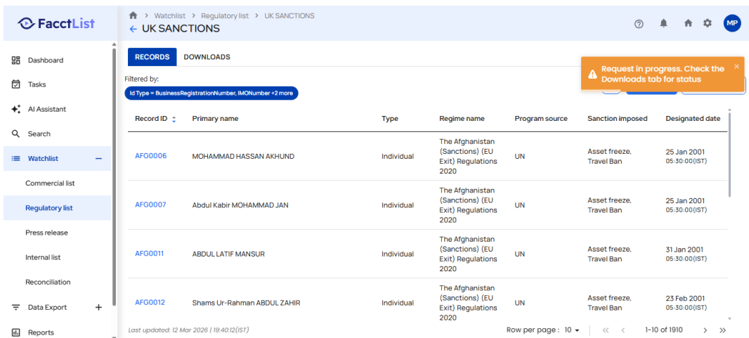
Screenshot: TestExecution_Step59_ACTION_Element.png
