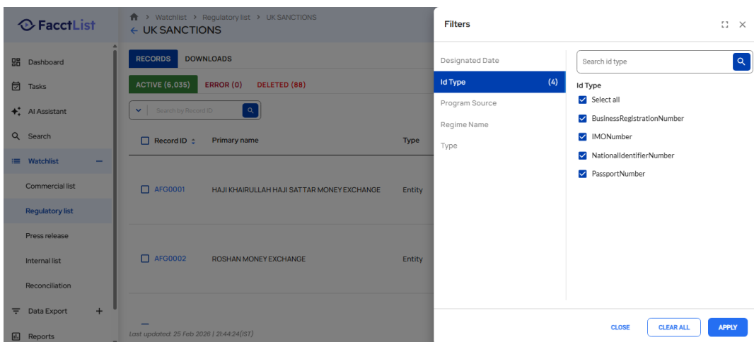
Screenshot: TestExecution_Step58_ACTION_Element.png
