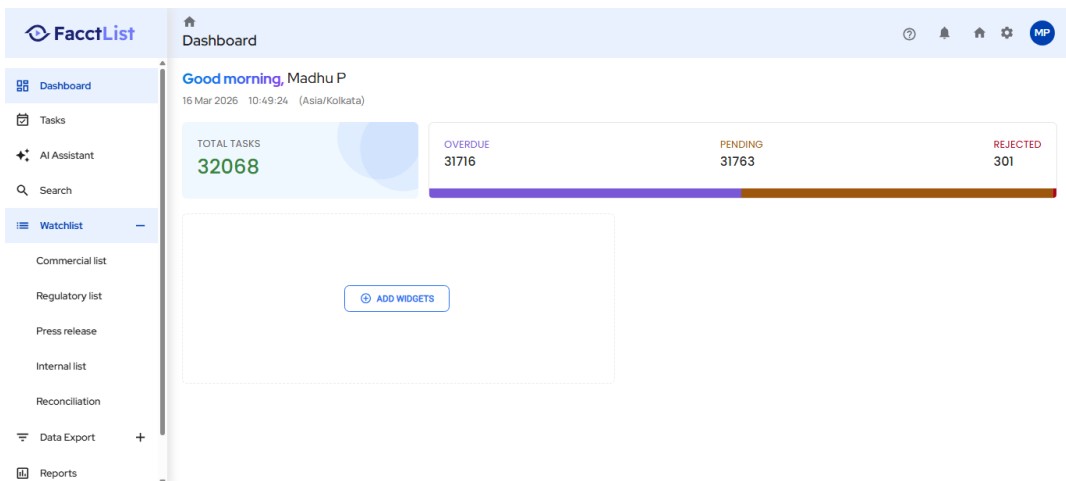
Screenshot: TestExecution_Step50_ACTION_Element.png
