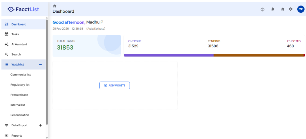
Screenshot: TestExecution_Step30_ACTION_Element.png
