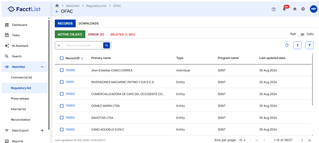
Screenshot: TestExecution_Step09_ACTION_Element.png
