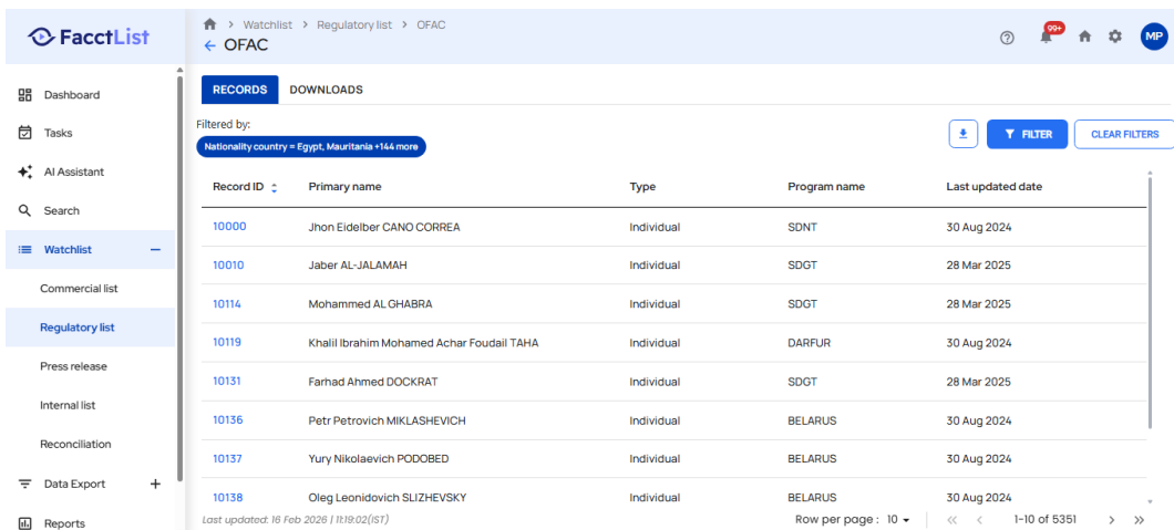
Screenshot: TestExecution_Step10_ACTION_Element.png
