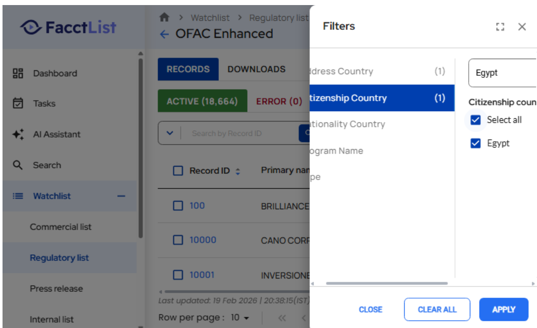
Screenshot: TestExecution_Step16_ACTION_Element.png
