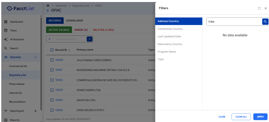
Screenshot: TestExecution_Step15_ACTION_Element.png
