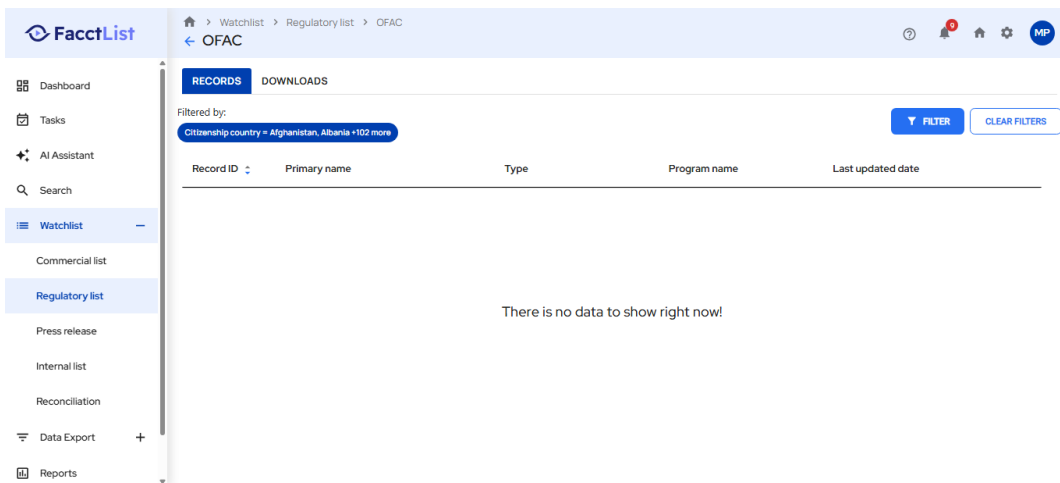
Screenshot: TestExecution_Step32_ACTION_Element.png
