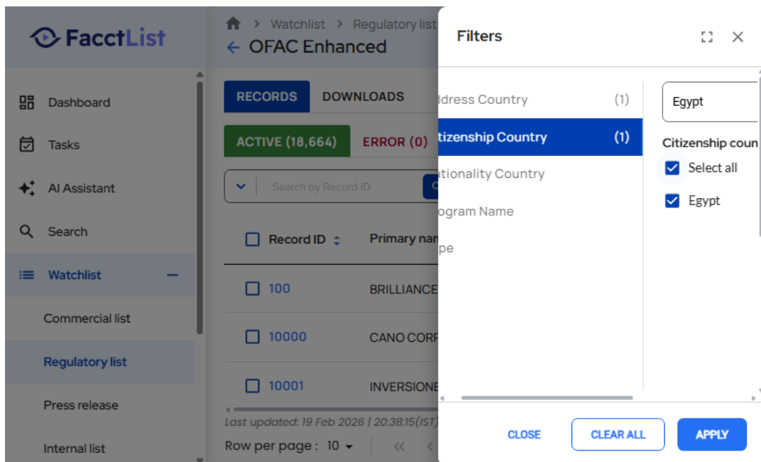
Screenshot: TestExecution_Step17_ACTION_Element.png
