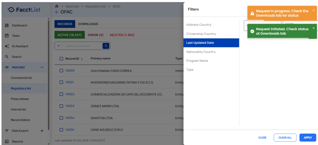
Screenshot: TestExecution_Step14_ACTION_Element.png
