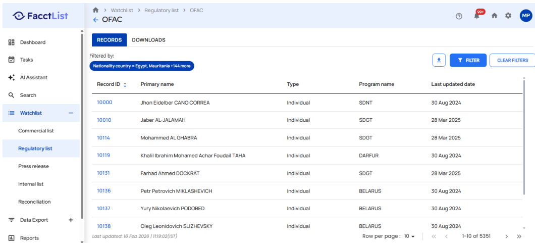
Screenshot: TestExecution_Step11_ACTION_Element.png
