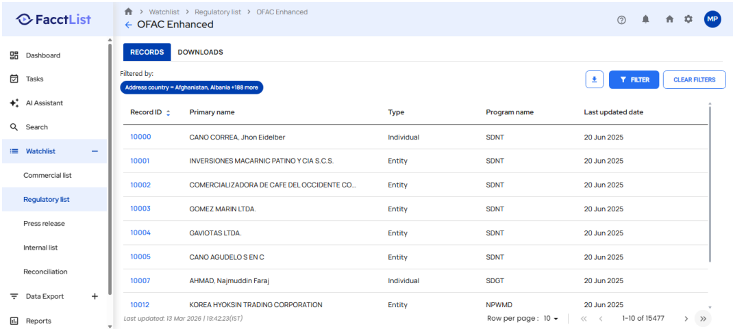
Screenshot: TestExecution_Step53_ACTION_Element.png
