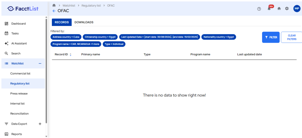
Screenshot: TestExecution_Step09_ACTION_Element.png
