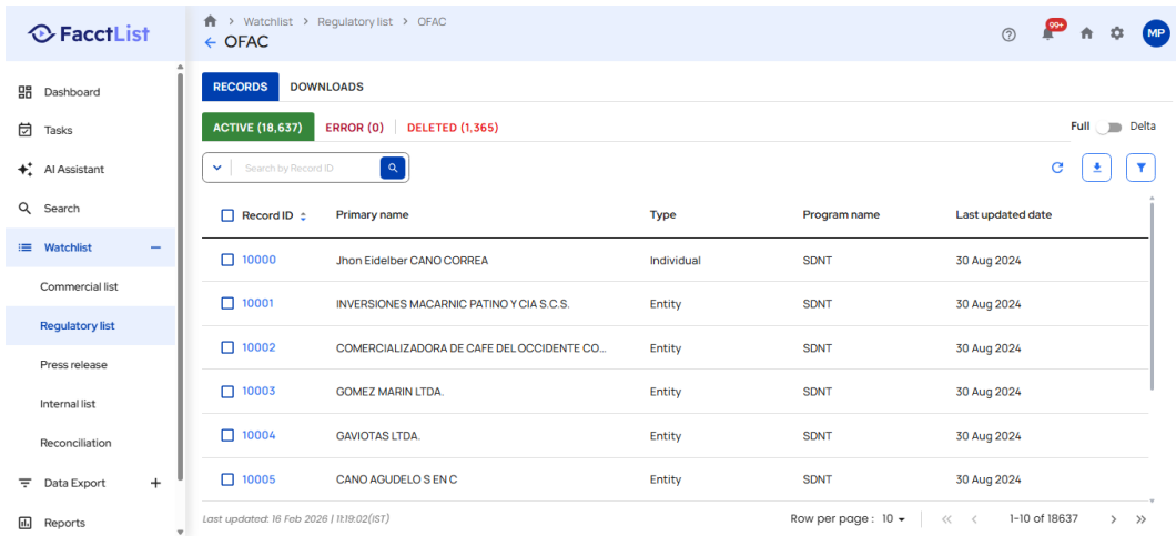
Screenshot: TestExecution_Step10_ACTION_Element.png
