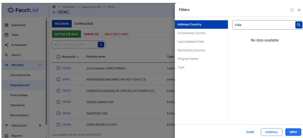
Screenshot: TestExecution_Step16_ACTION_Element.png
