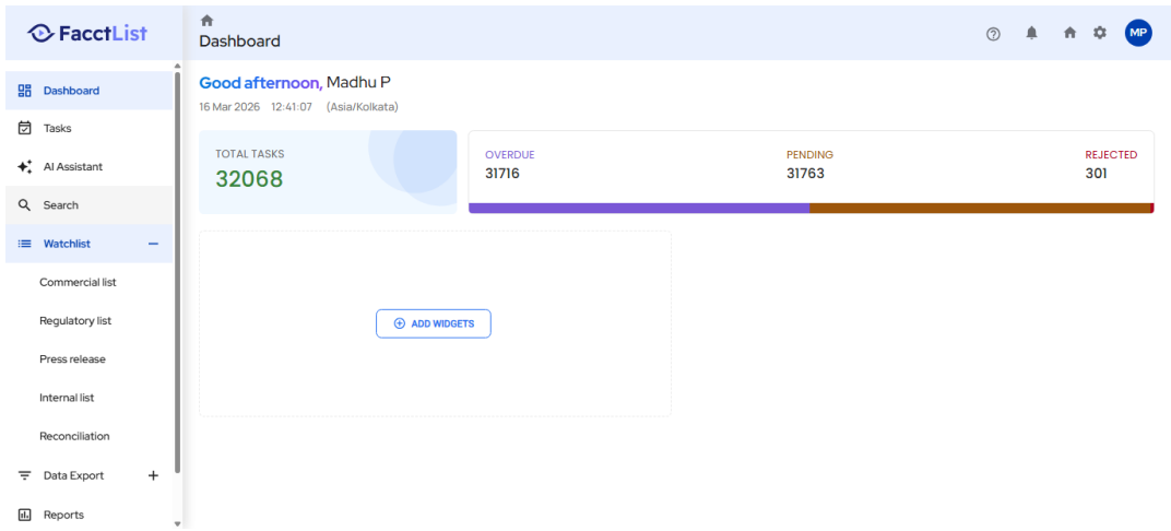
Screenshot: TestExecution_Step54_ACTION_Element.png
