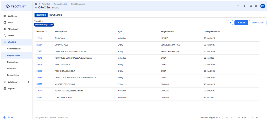
Screenshot: TestExecution_Step49_ACTION_Element.png
