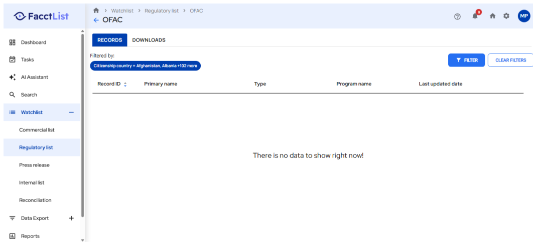
Screenshot: TestExecution_Step25_ACTION_Element.png
