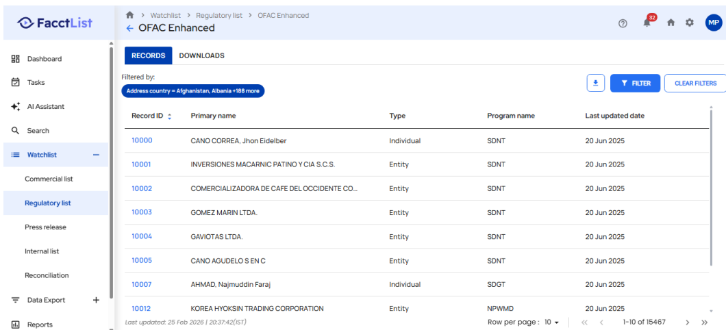
Screenshot: TestExecution_Step29_ACTION_Element.png
