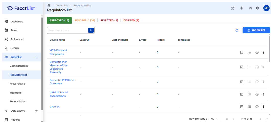
Screenshot: TestExecution_Step49_ACTION_Element.png
