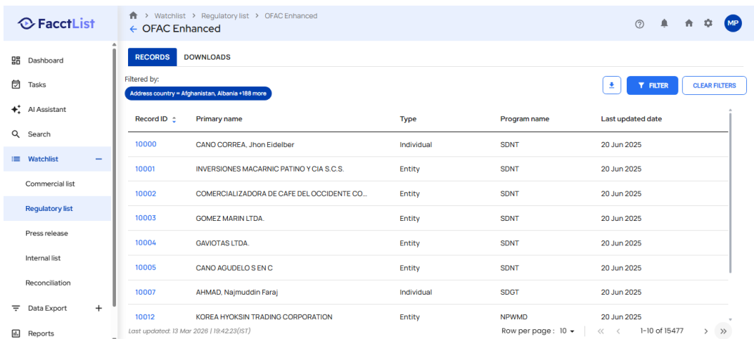
Screenshot: TestExecution_Step47_ACTION_Element.png
