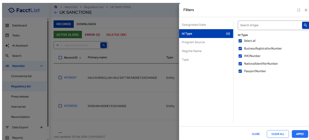
Screenshot: TestExecution_Step51_ACTION_Element.png
