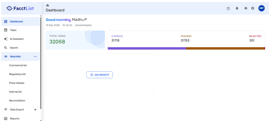
Screenshot: TestExecution_Step48_ACTION_Element.png
