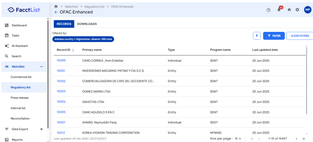
Screenshot: TestExecution_Step30_ACTION_Element.png
