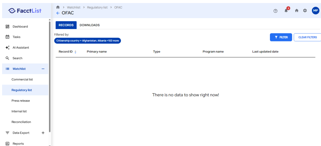
Screenshot: TestExecution_Step27_ACTION_Element.png
