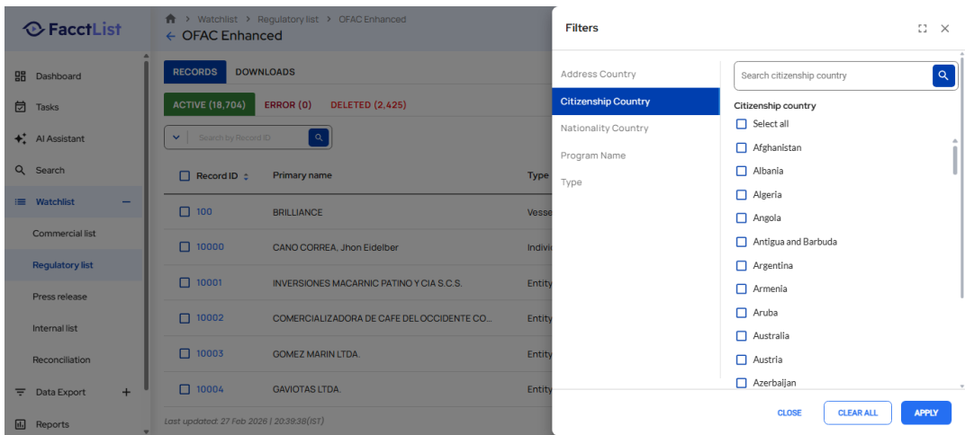
Screenshot: TestExecution_Step46_ACTION_Element.png
