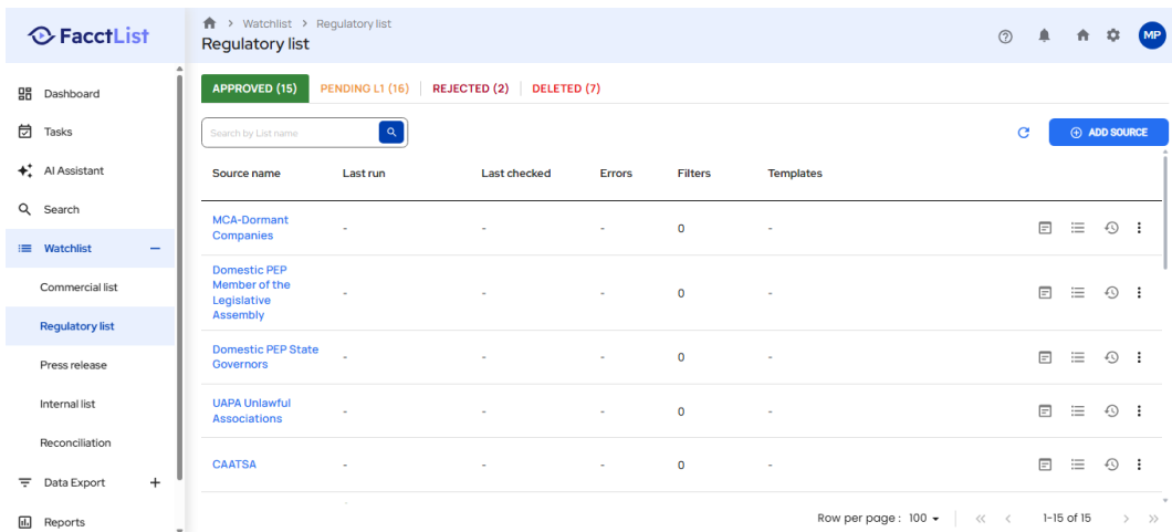
Screenshot: TestExecution_Step40_ACTION_Element.png
