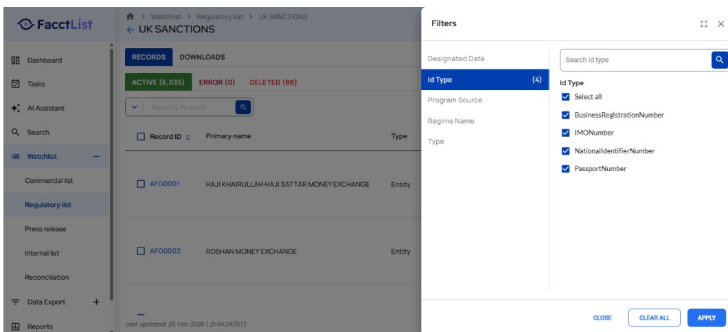
Screenshot: TestExecution_Step42_ACTION_Element.png
