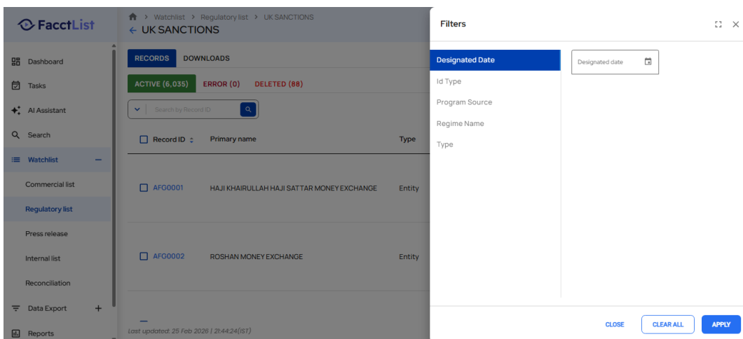
Screenshot: TestExecution_Step41_ACTION_Element.png
