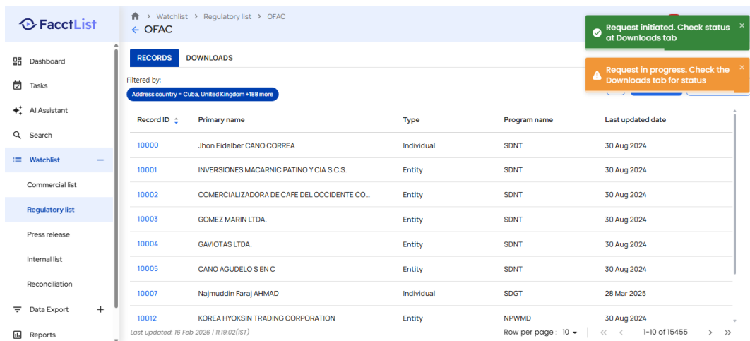
Screenshot: TestExecution_Step08_ACTION_Element.png
