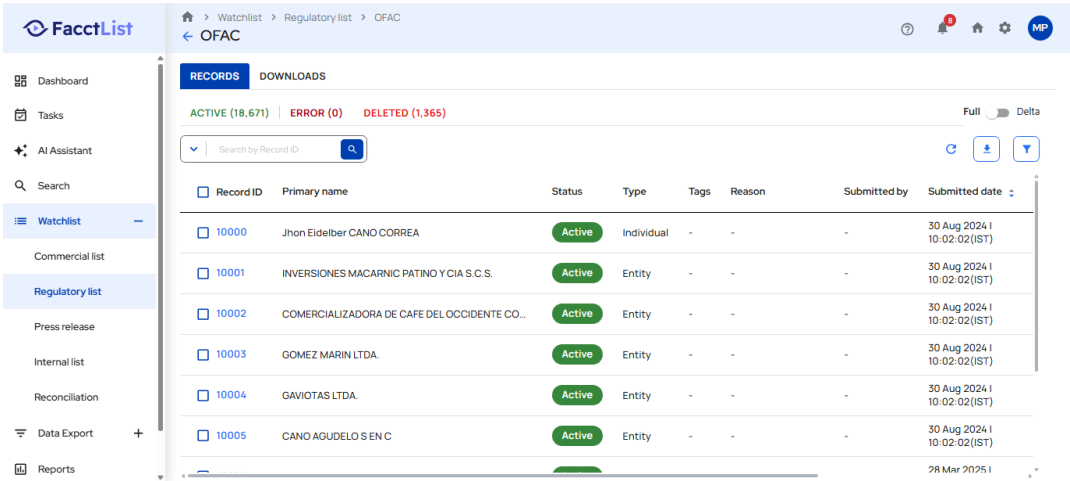
Screenshot: TestExecution_Step24_ACTION_Element.png
