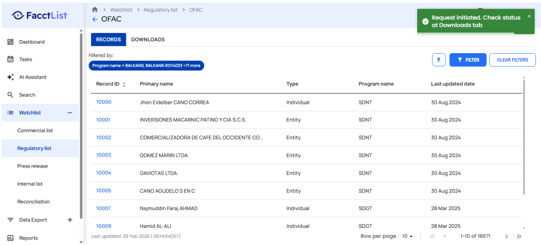
Screenshot: TestExecution_Step23_ACTION_Element.png
