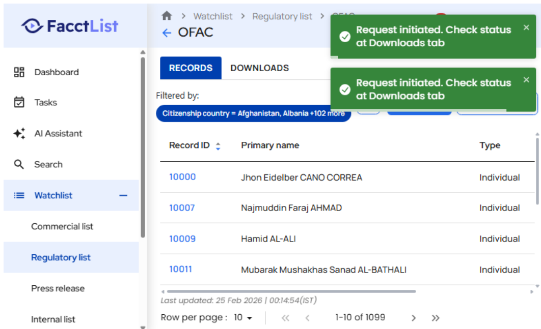
Screenshot: TestExecution_Step17_ACTION_Element.png
