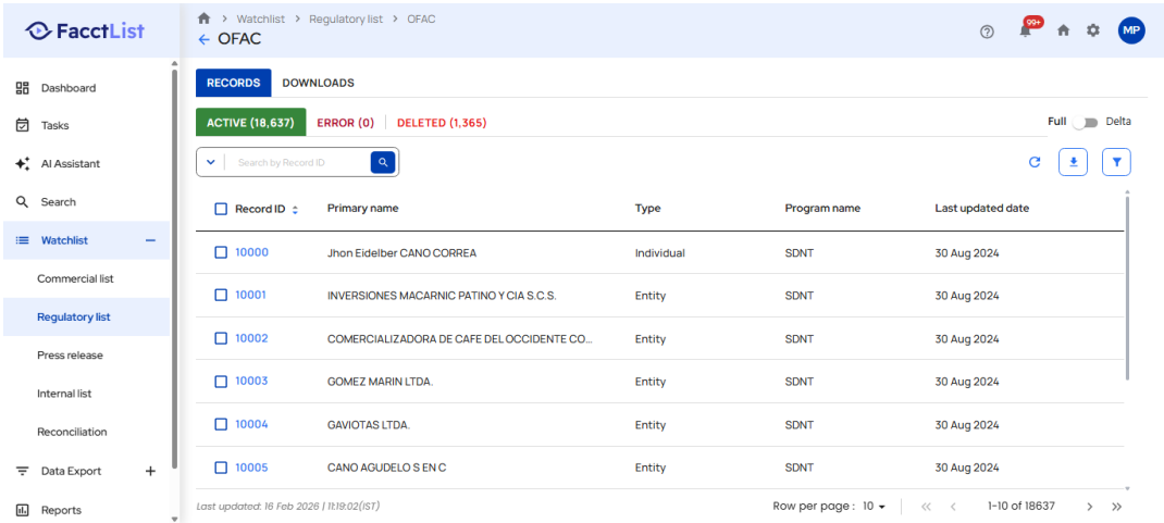
Screenshot: TestExecution_Step04_ACTION_Element.png
