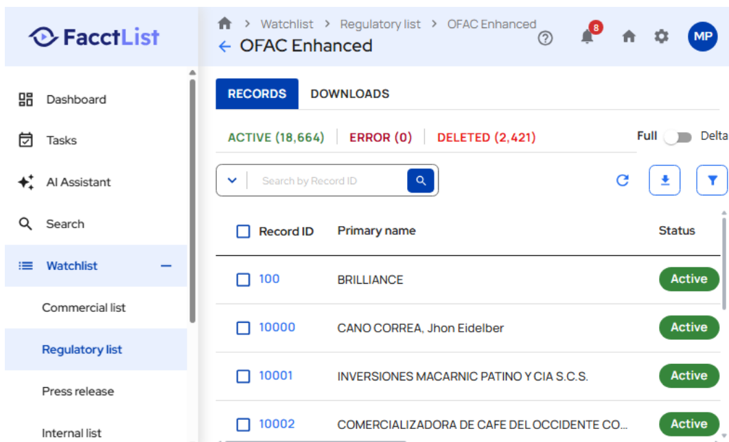
Screenshot: TestExecution_Step15_ACTION_Element.png
