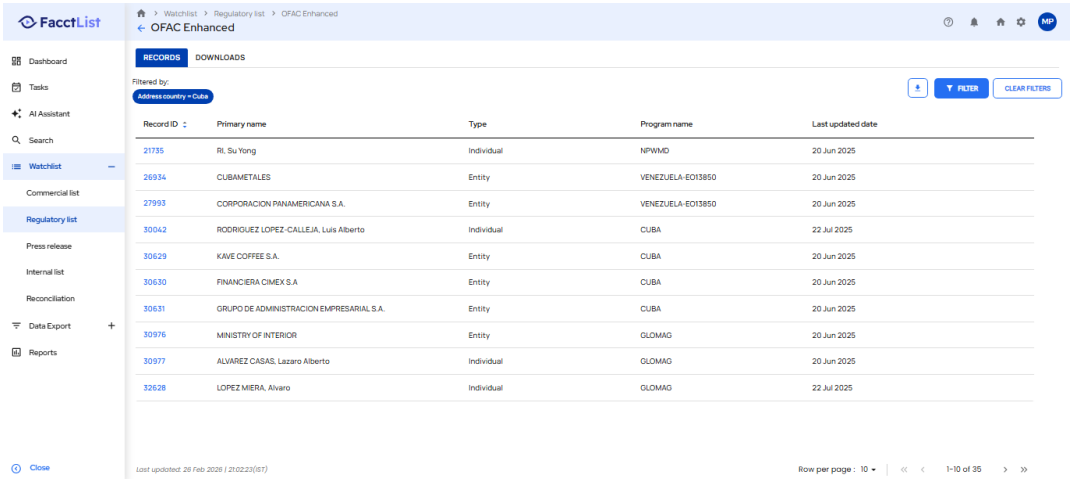
Screenshot: TestExecution_Step38_ACTION_Element.png
