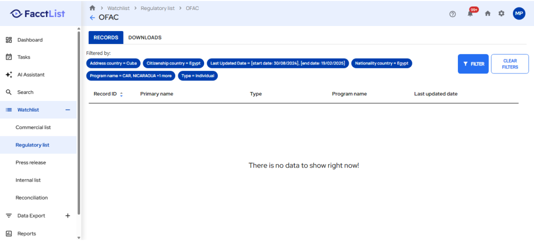
Screenshot: TestExecution_Step03_ACTION_Element.png
