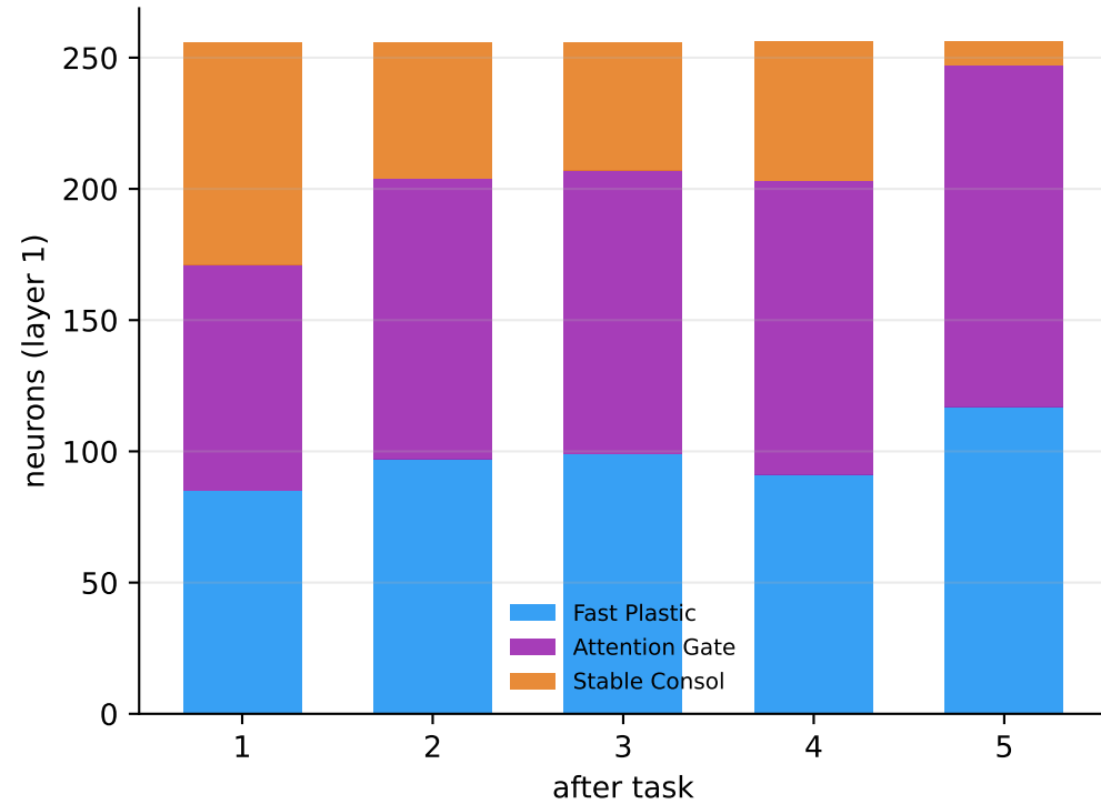
Functional memory roles evolve across tasks
