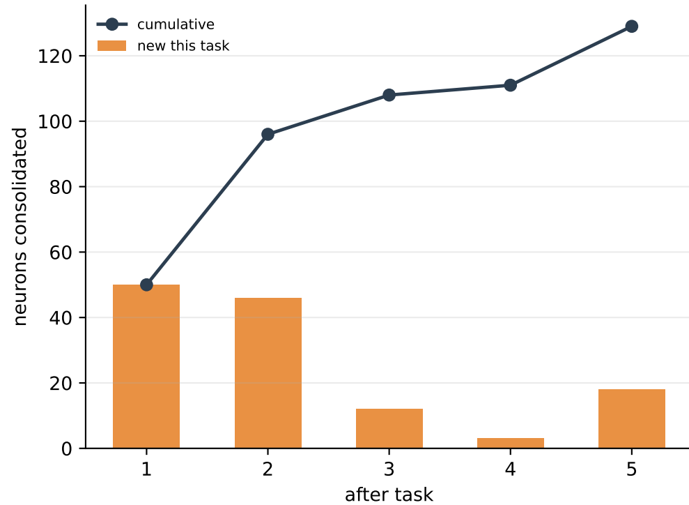
STM → LTM transitions
