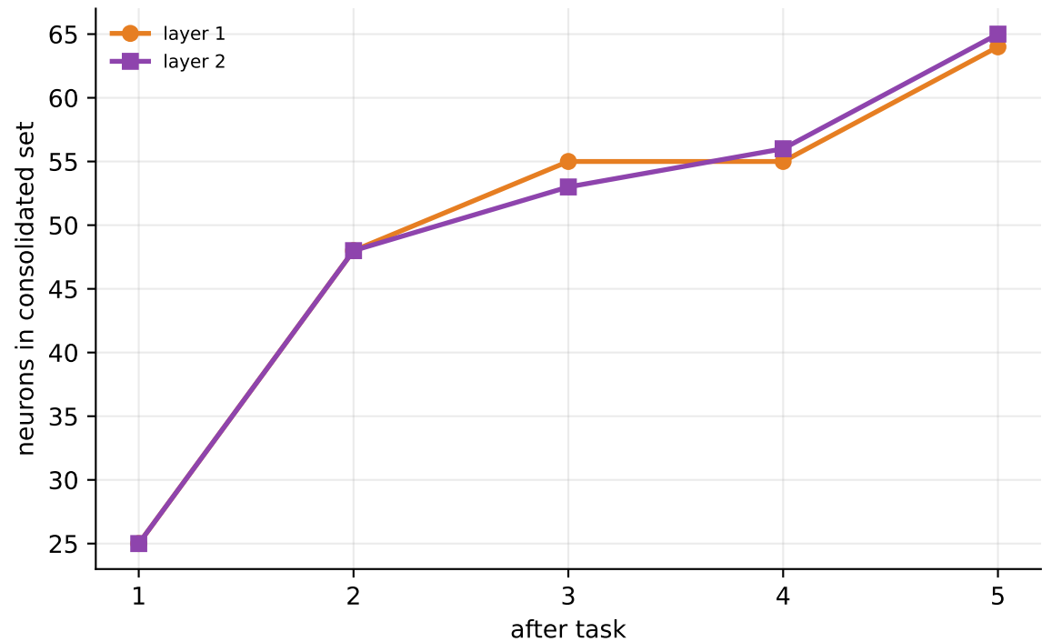
Growth of the consolidated (LTM) set
