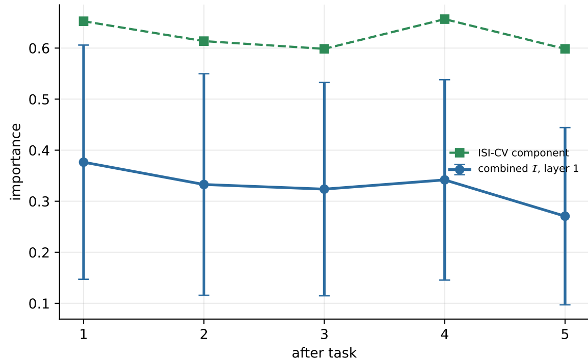
Combined importance and its spiking component
