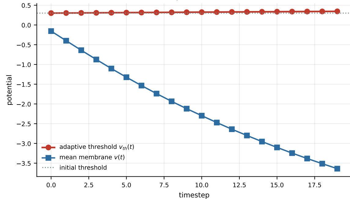
Threshold adapts as the network fires
