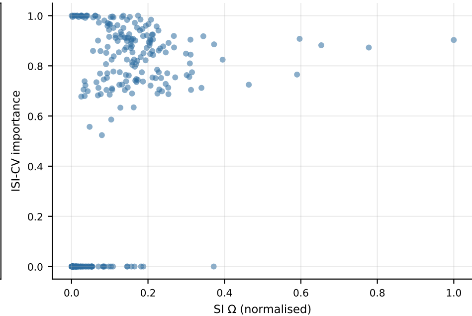
Gradient vs spiking importance ( r = 0.413 )
