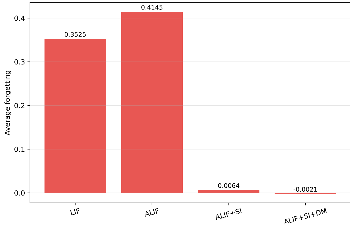
Average forgetting (lower is better)
