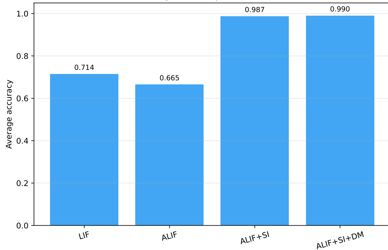
Average accuracy after all tasks
