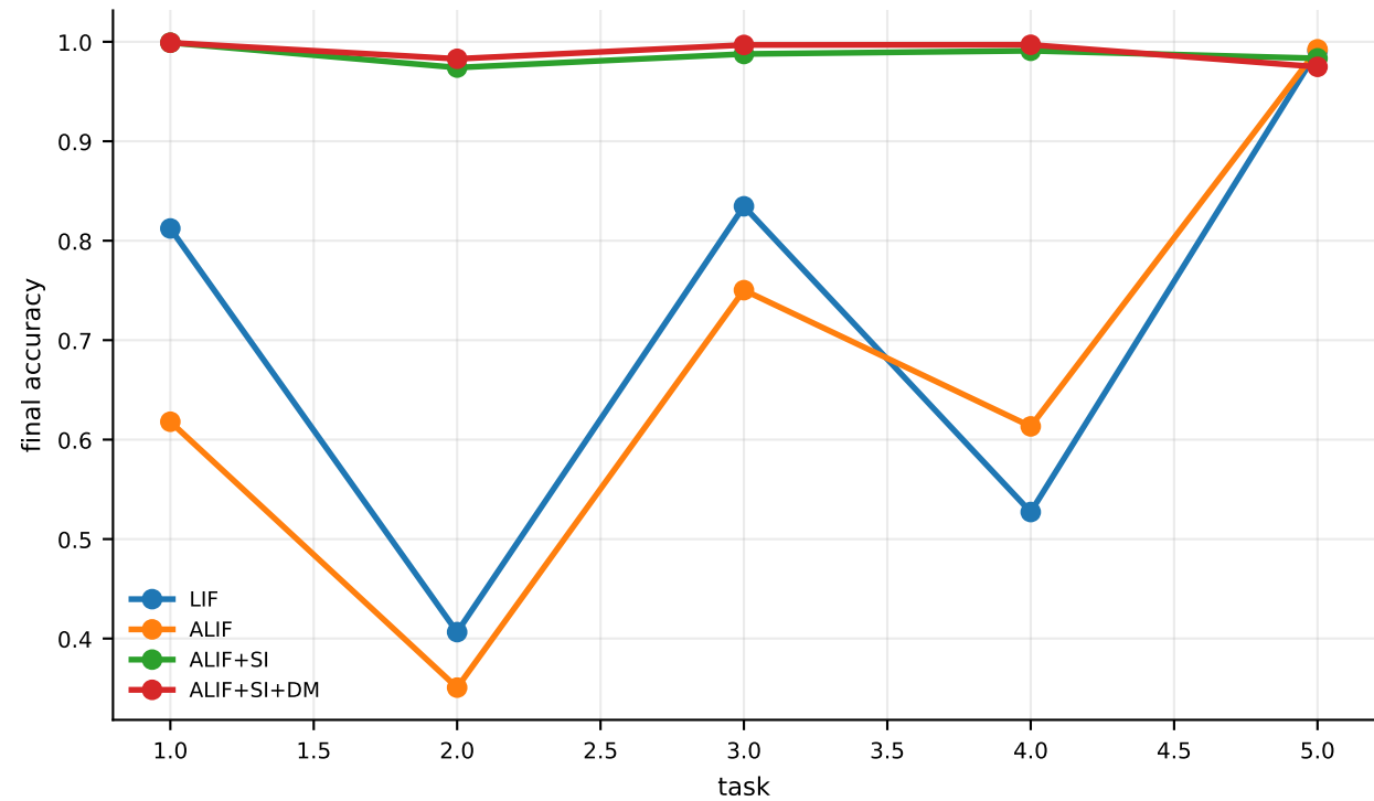
Final accuracy per task
