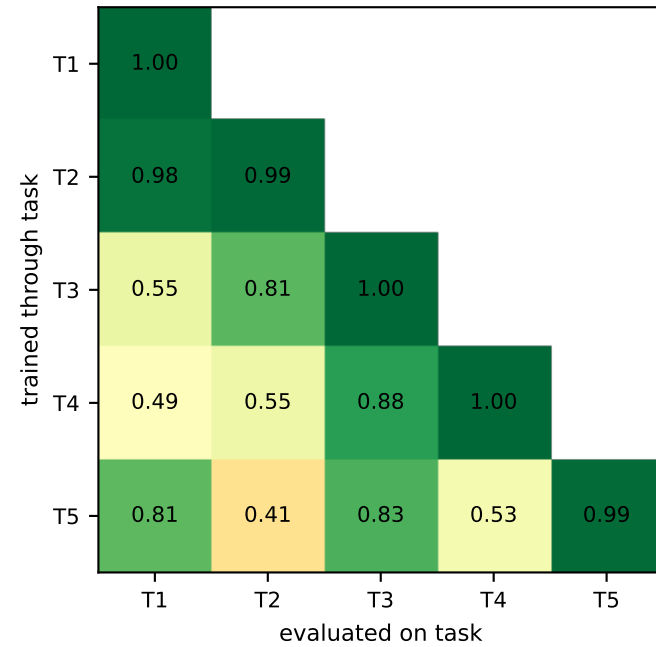
LIF
