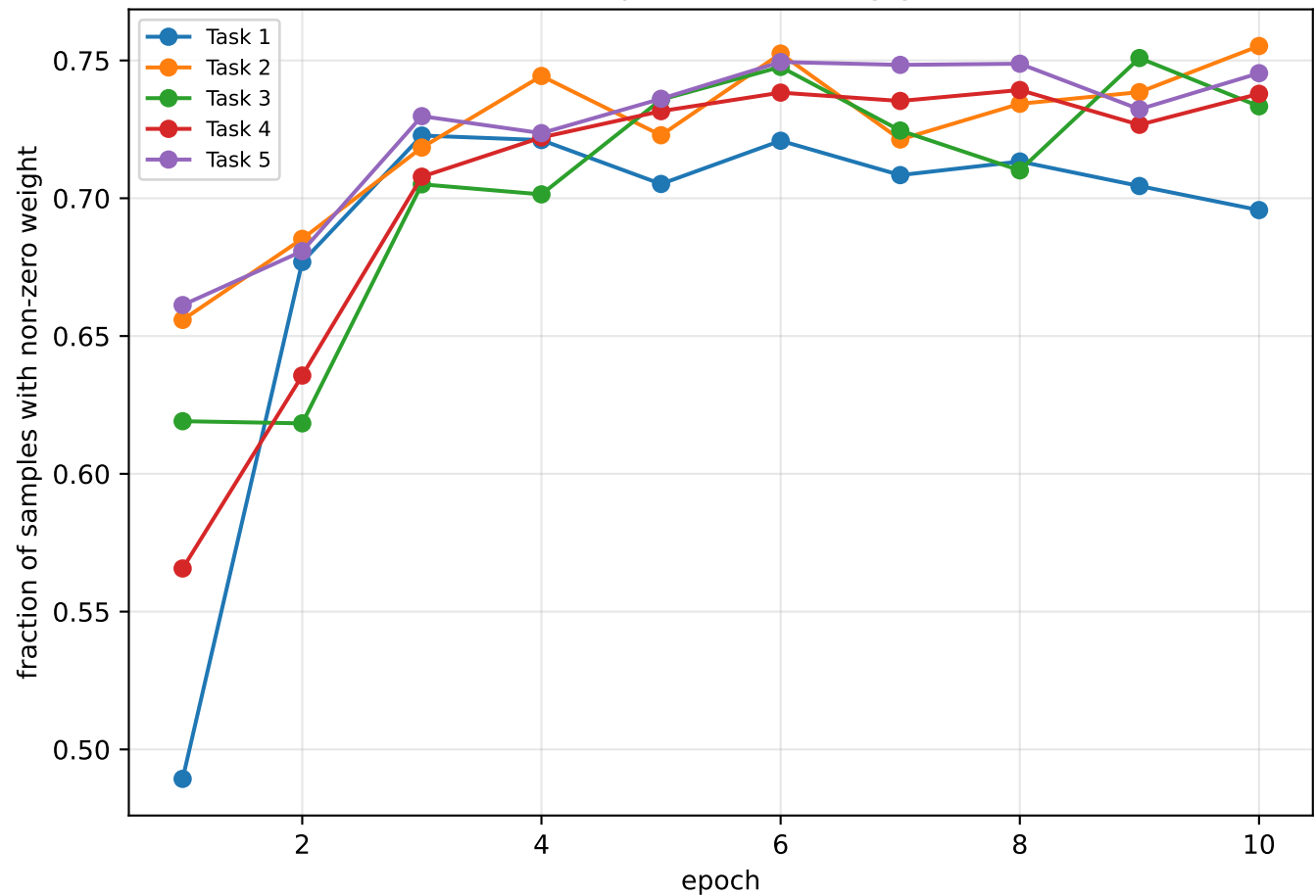
Share of samples contributing gradient
