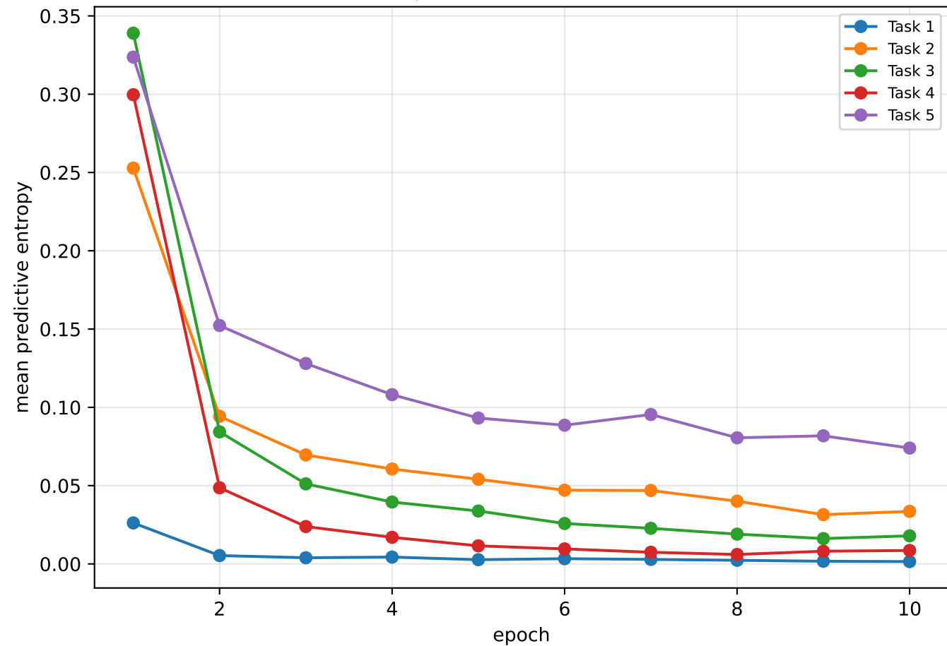
Uncertainty falls as each task is learned
