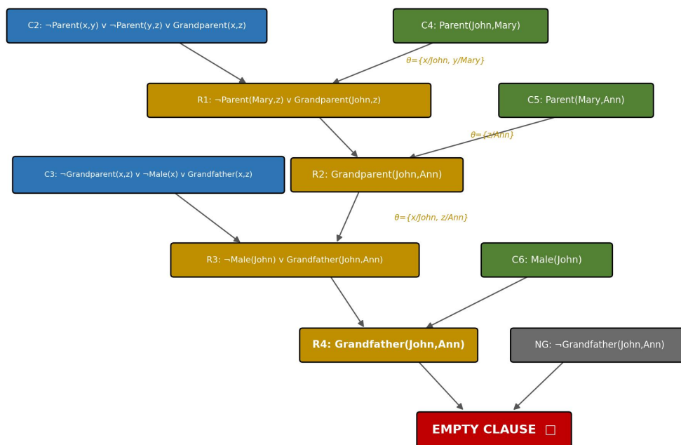
Q4 — First-Order Resolution Proof Tree (Family Domain)
