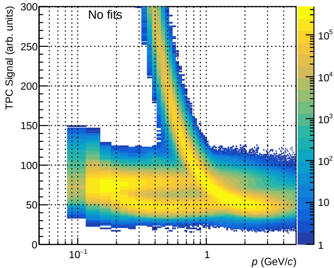
TPC dE/dx - Pb-Pb 2023, V0 skim (all runs)
