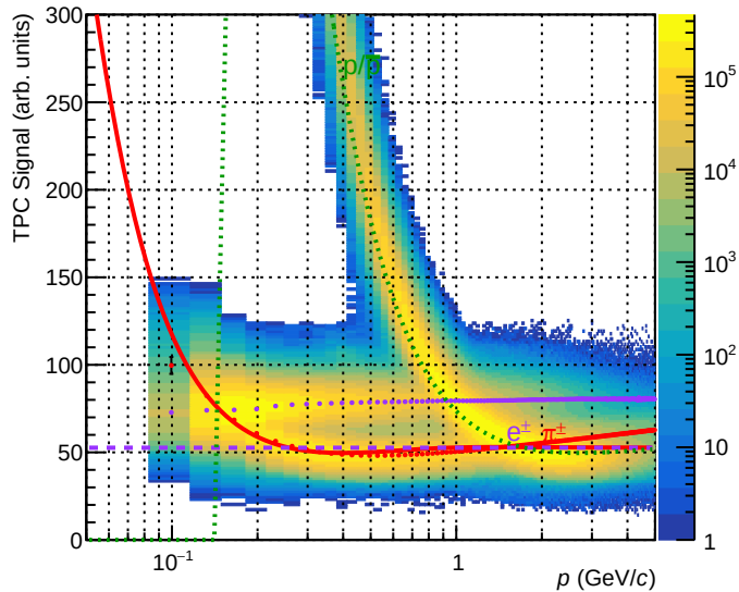
TPC dE/dx - Pb-Pb 2023, V0 skim + BB curves
