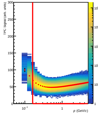
Pions (V0: K_s^0 \rightarrow \pi^+\pi^- )
