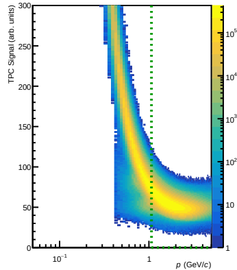
Proton (V0: \Lambda \rightarrow p\pi^- )
