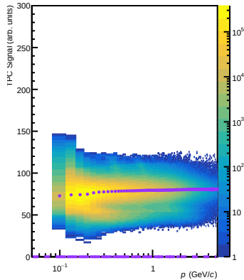
Electrons (V0: \gamma \rightarrow e^+e^- )
