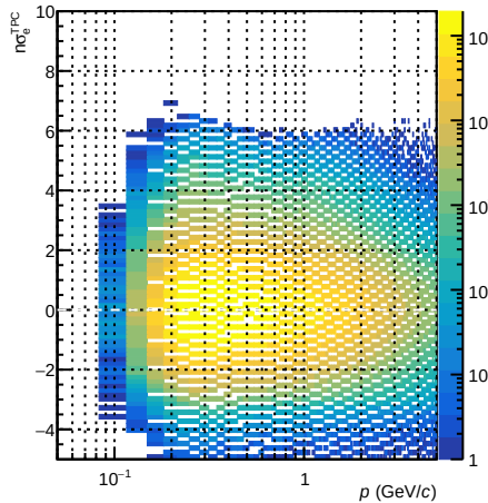
TPC n\sigma_e - V0 pions
