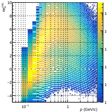
TPC n\sigma_e - V0 electrons
