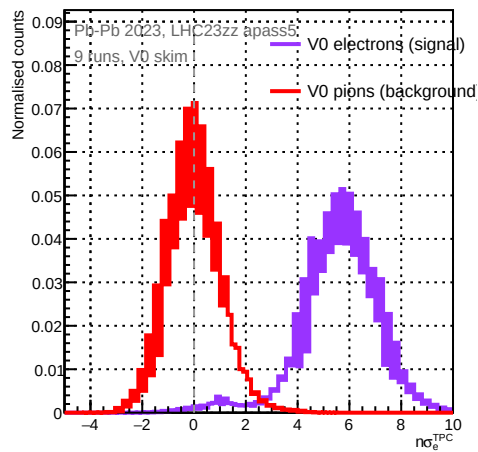
n\sigma_e^{\text{TPC}} at p = 0.9-1.1 GeV/c
