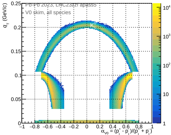
Armenteros-Podolanski - All V0 tracks
