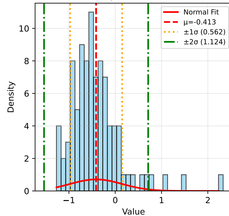
b6 (n=93, \mu=-0.413 , \sigma=0.562 )
