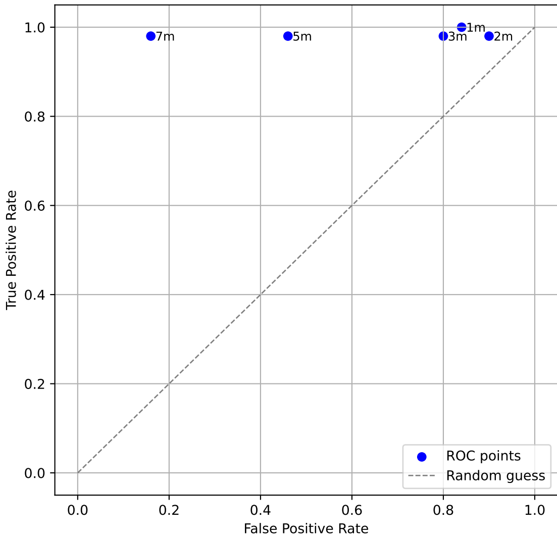
ROC Curve
