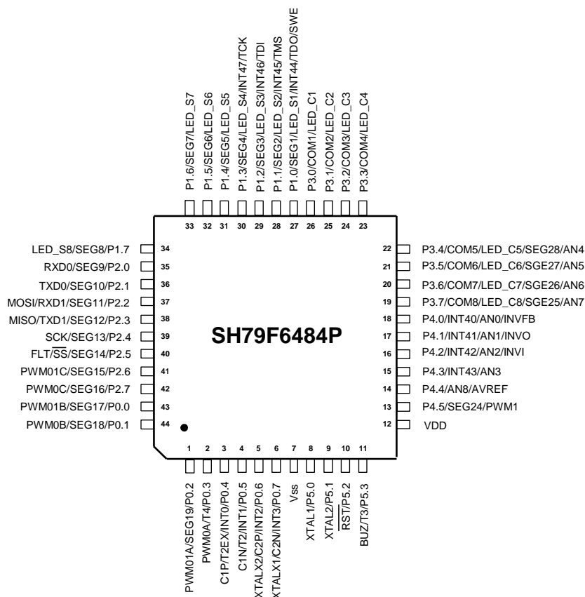
Pin Configuration Diagram LQFP44
