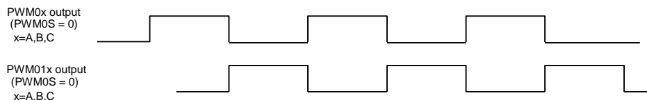
PWM0 and PWM01 output waveform
