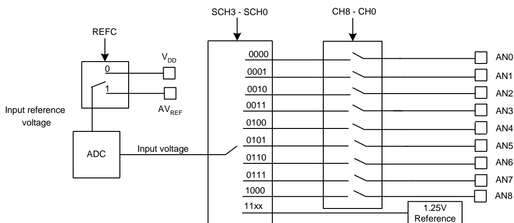
ADC Diagram
