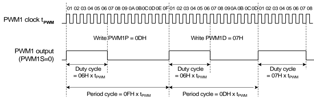
PWM1 output Period or Duty cycle changing example
