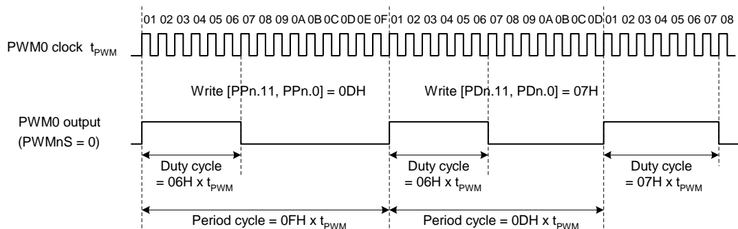
PWM0 output Period or Duty cycle changing example
