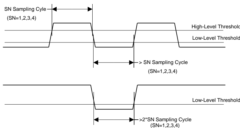
External Interrupt Detecting
