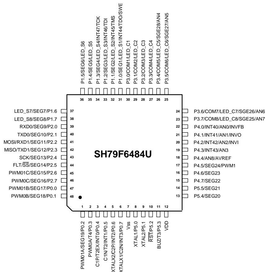
Pin Configuration Diagram TQFP48
