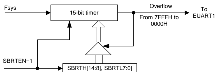
Baudrate Generator for EUART
