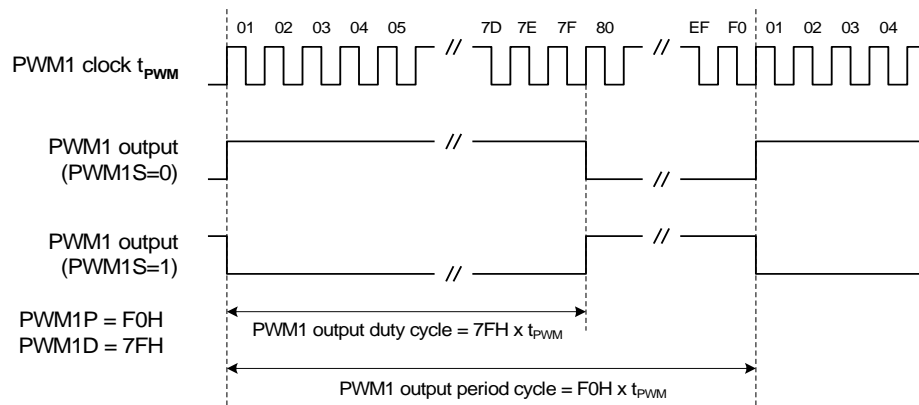
PWM1 output example
