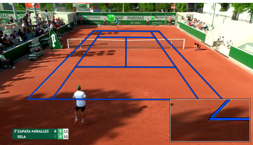
No-Bells-Just-Whistles
