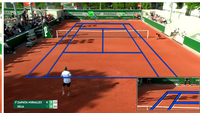
KaliCalib
