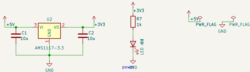
3.3 V regulator (USB 5 V -> AMS1117-3.3 -> 3V3)
