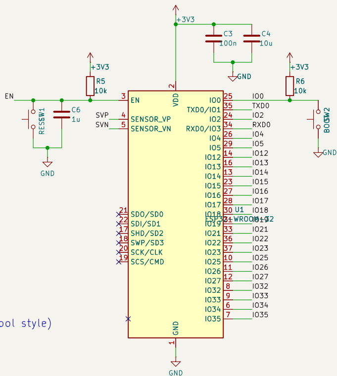
ESP32-WROOM-32 (EN/BOOT buttons, 3V3 decoupling)
