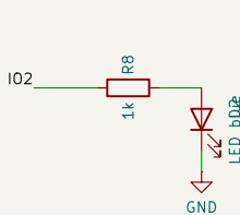
User LED (IO2)
