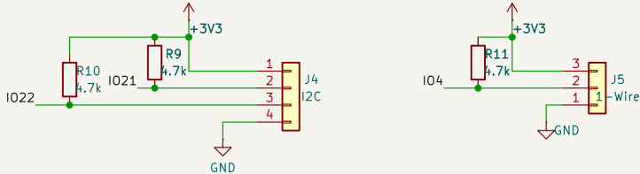
I2C header (IO21 SDA / IO22 SCL, 4k7 puW headers (DS18B20 pinout: GND, DQ, 3V3)
