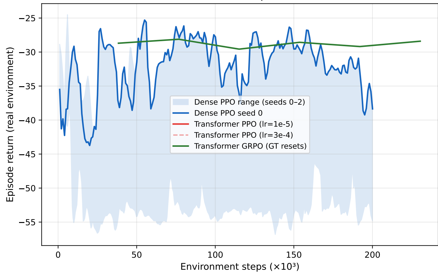
Part 2 — All methods comparison (real env)
