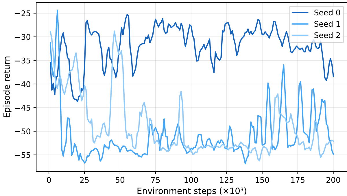
Part 1 — Dense PPO (3 seeds)
