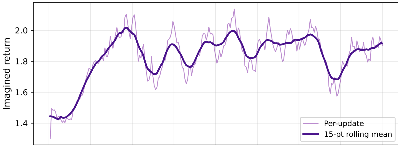
Part 2d — GRPO with DreamerV3 World Model
