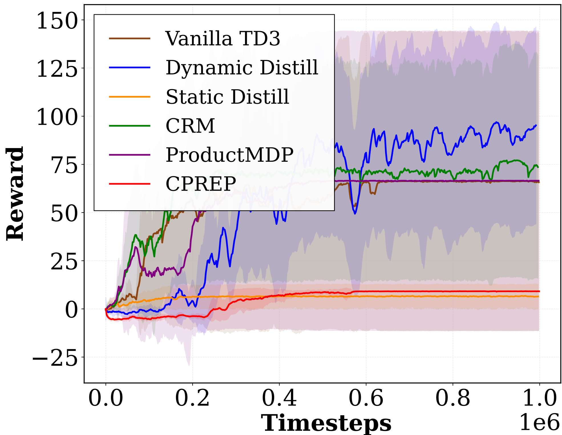
FlatWorld Sequence
