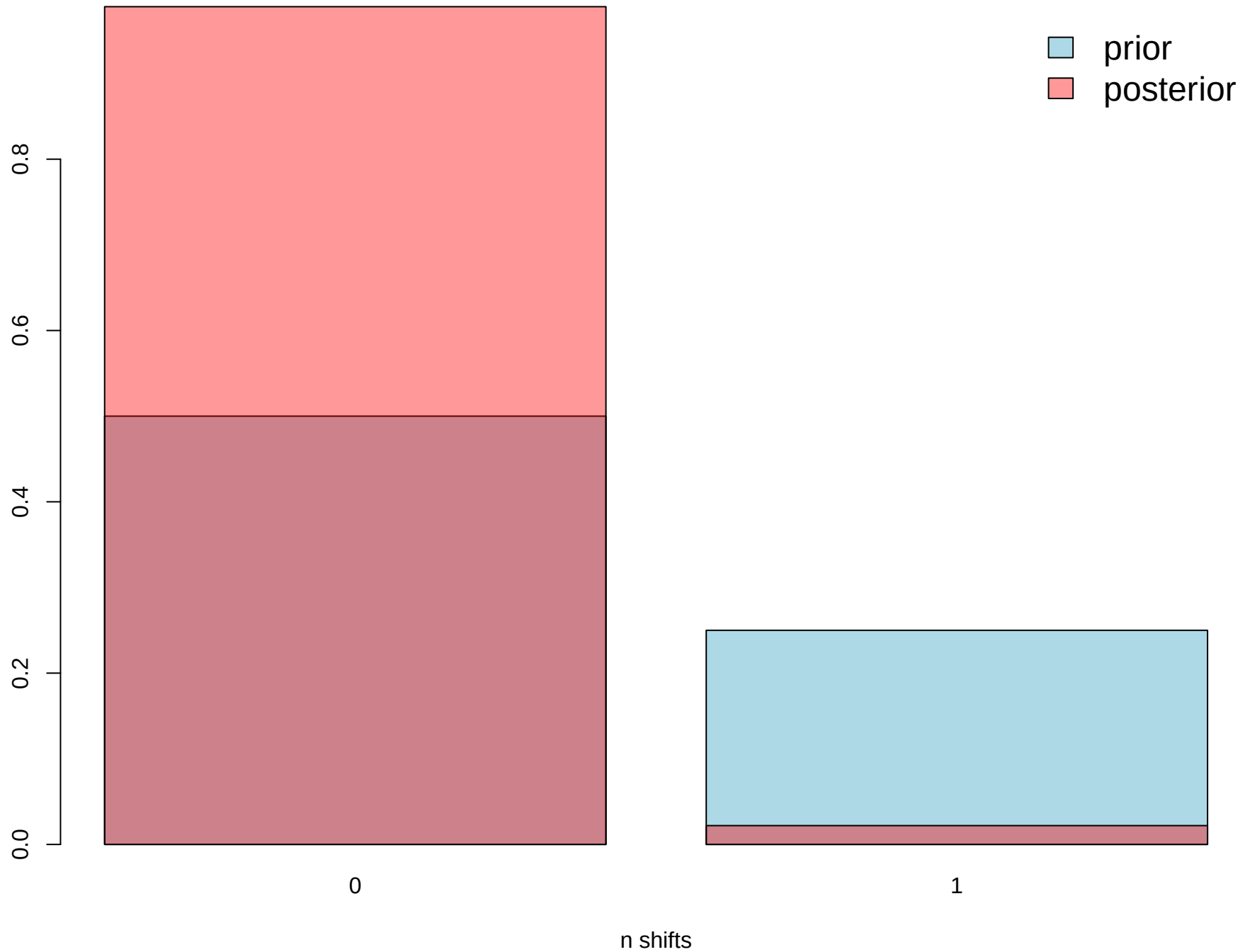
Comparison prior/posterior distributions of the number of shifts
