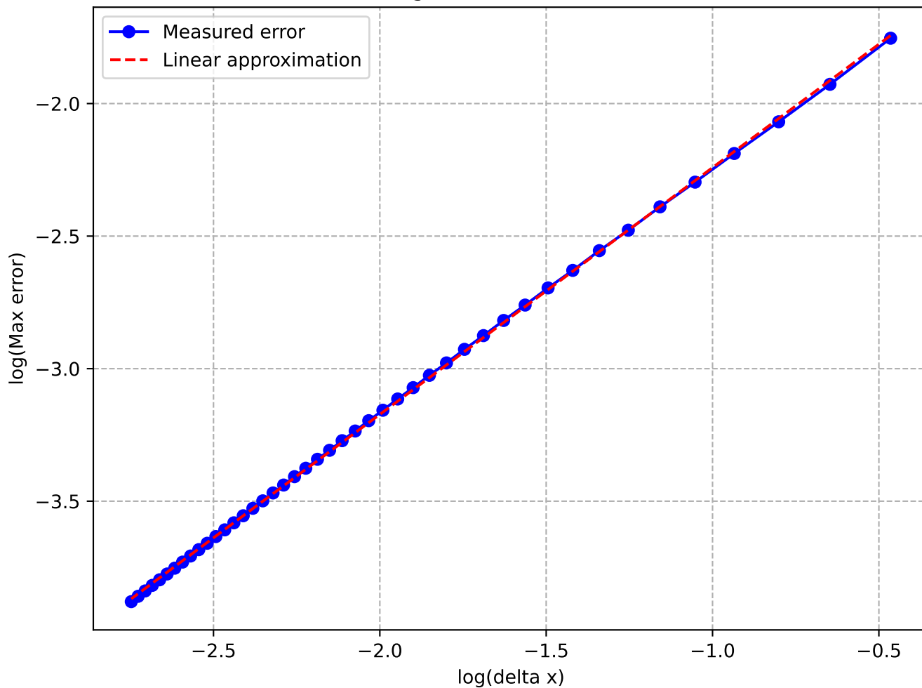
Convergence and method order
