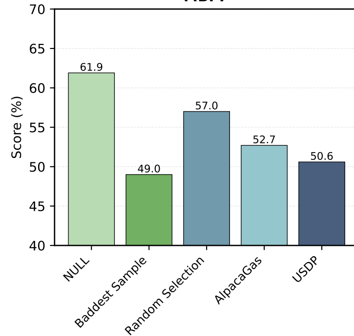
MBPP
