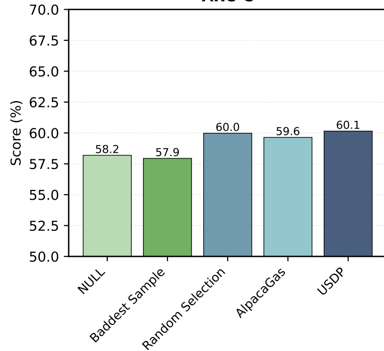
ARC-C
