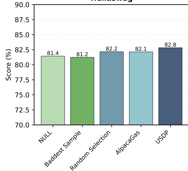
Hellaswag
