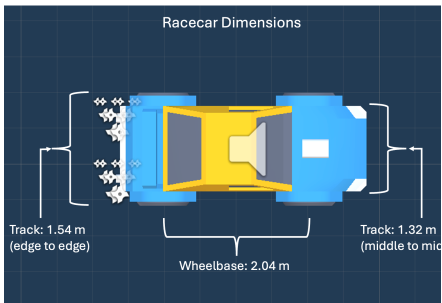
Figure 1: Racecar dimensions: wheelbase and track width.
