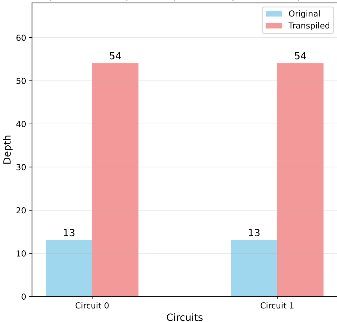
Original vs Transpiled Depth Side-by-Side Comparison
