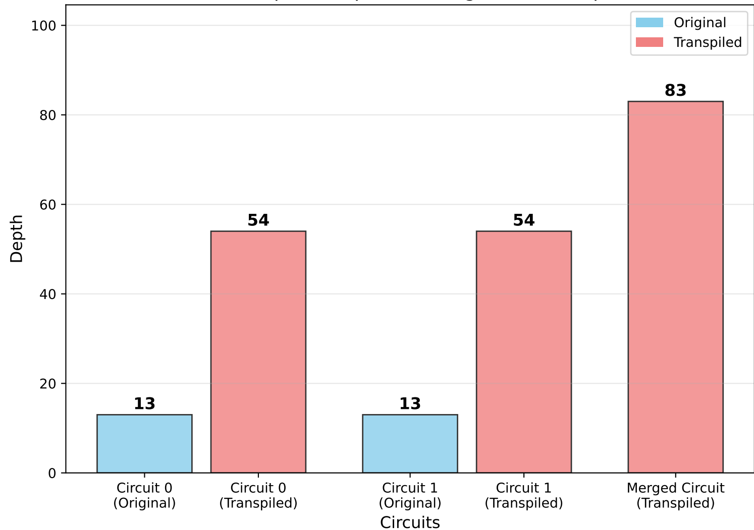
Circuit Depth Comparison: Original vs Transpiled
