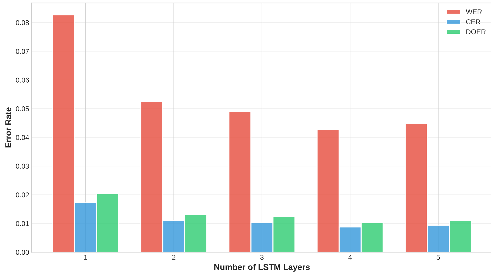
Sequence Labeling Performance - Val Dataset
