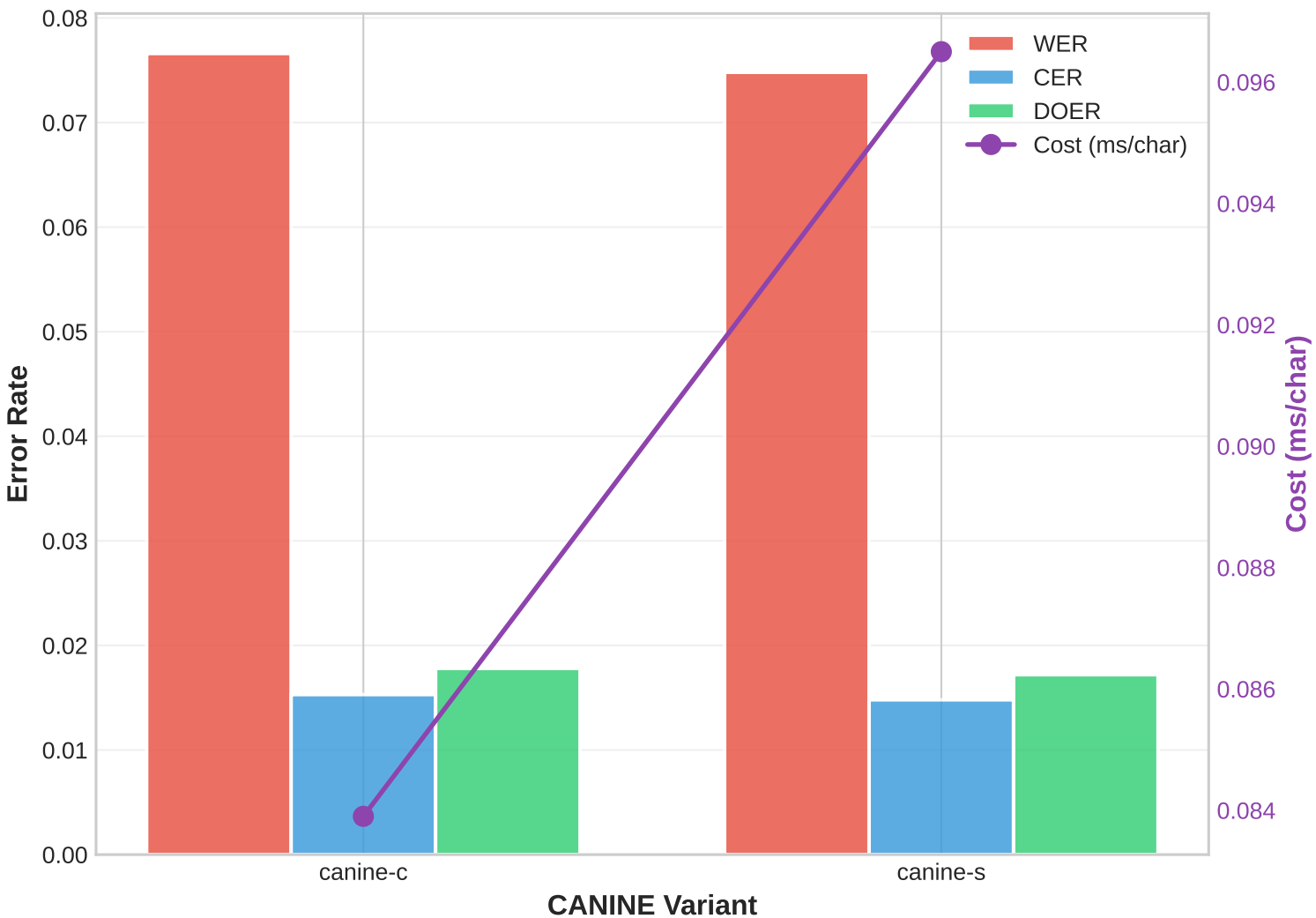
CANINE Performance - Test Dataset
