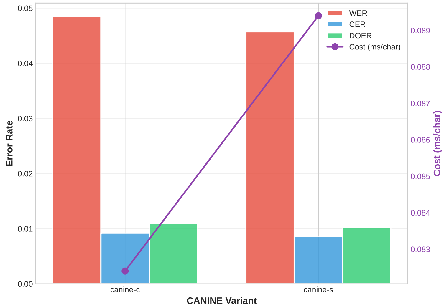
CANINE Performance - Val Dataset
