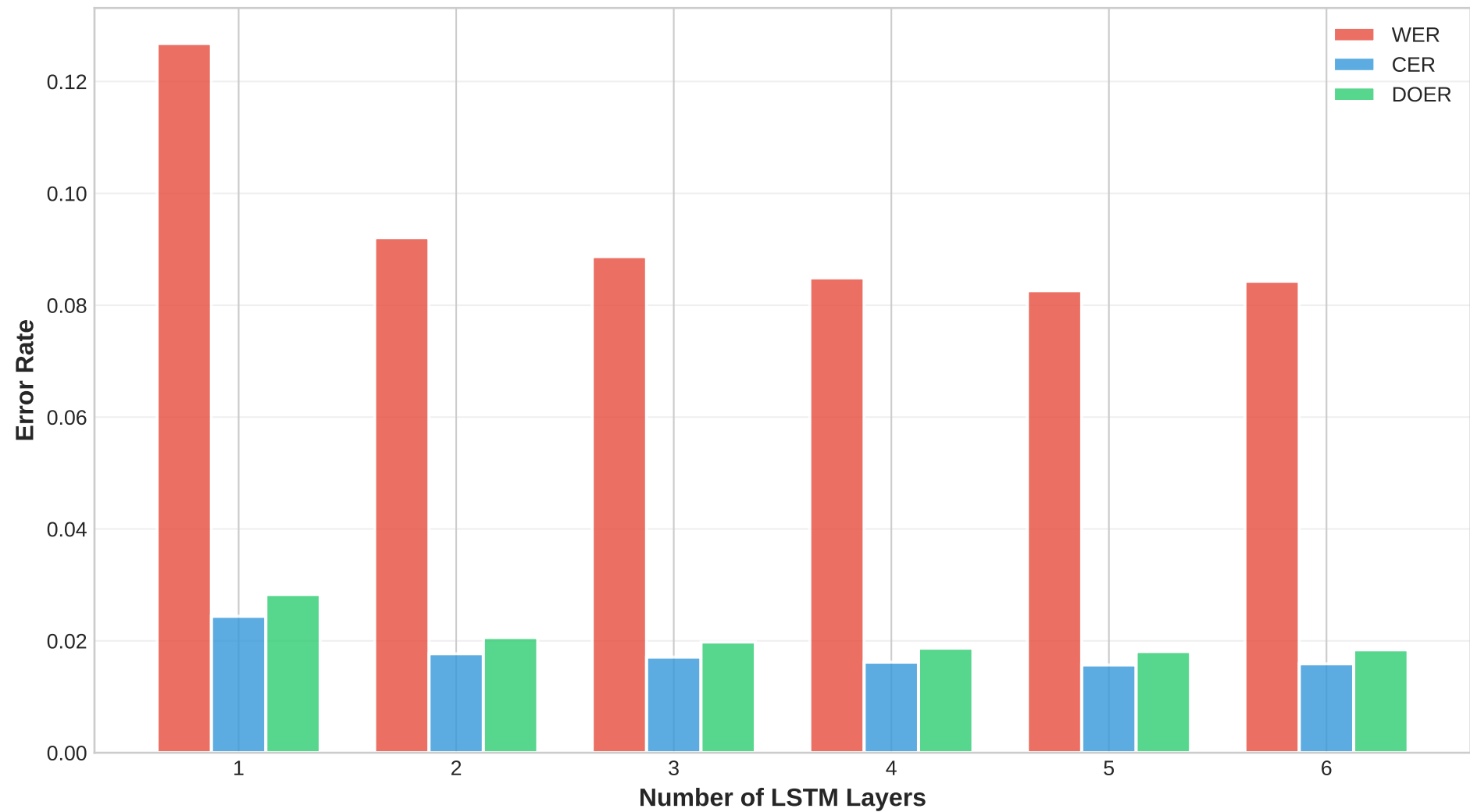
Sequence Labeling Performance - Test Dataset
