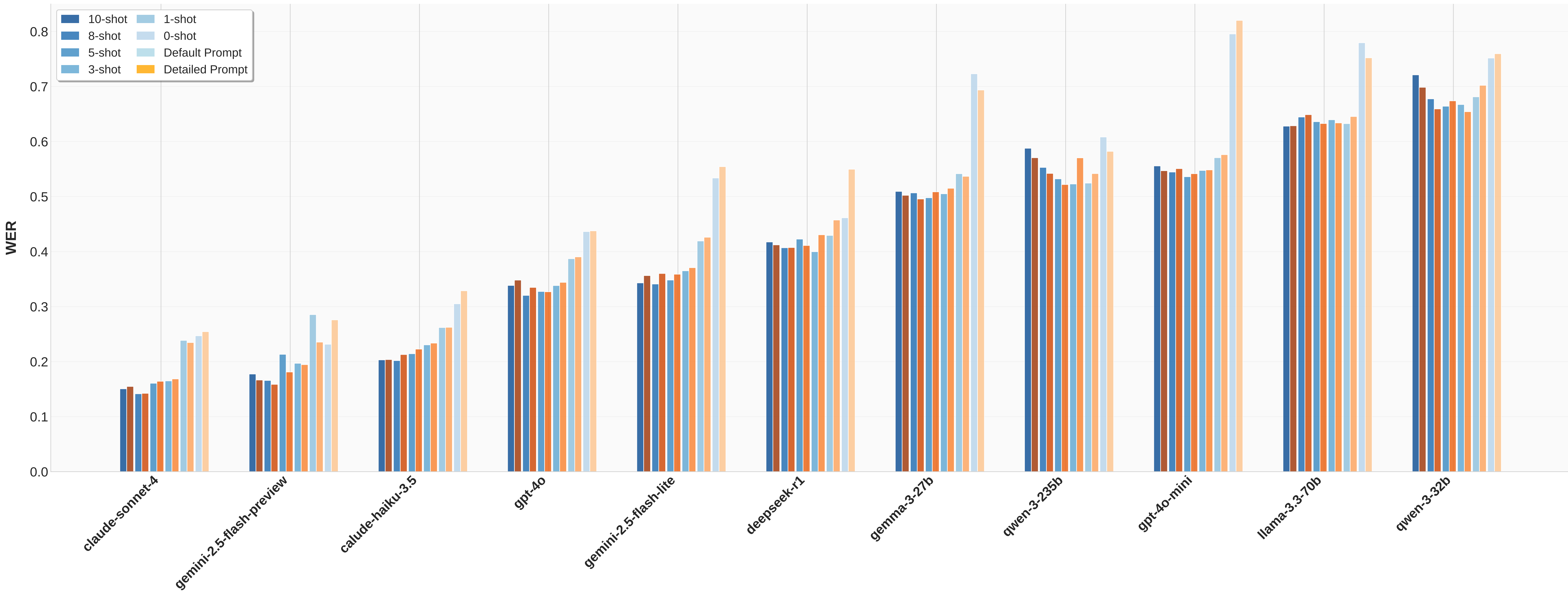
Model Performance: WER by Few-shot Configuration and Prompt Style
