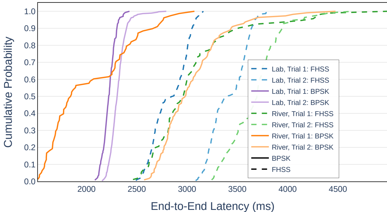
Cumulative Distribution Function of End-to-End Latency
